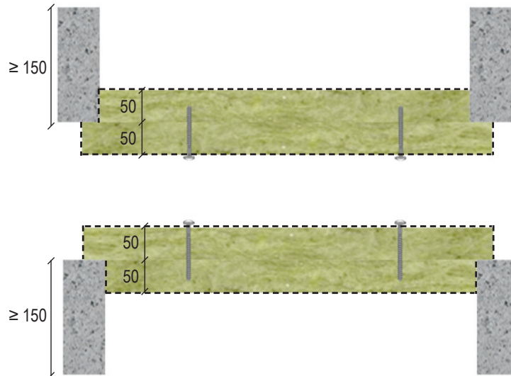
Rigid floor
